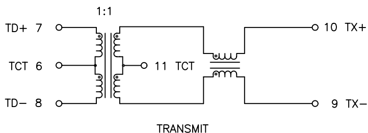
SCHEMATIC
