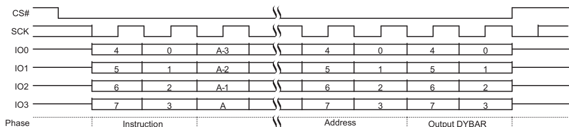
Figure 104. DYBRD QPI Mode Command Sequence
