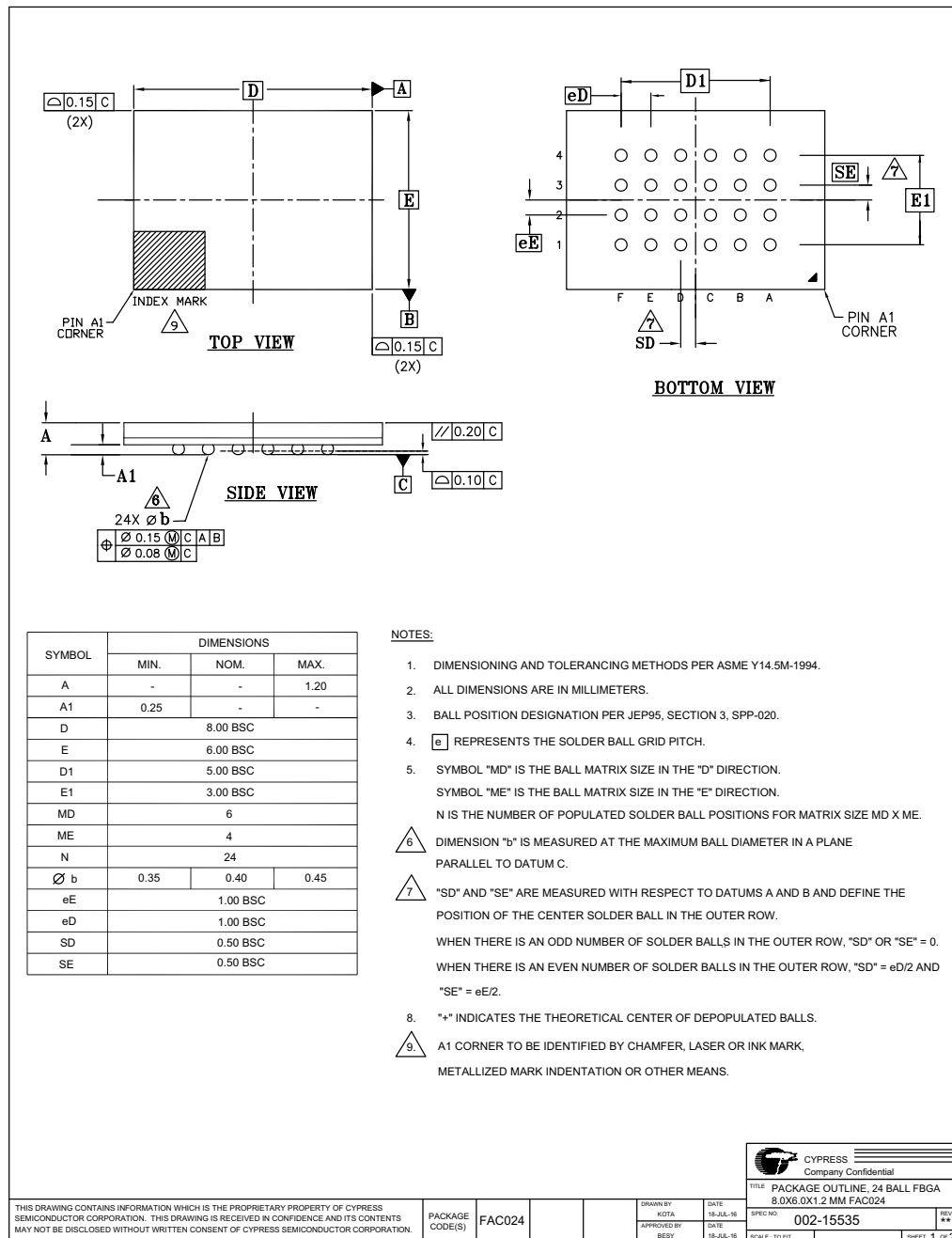
Figure 45. Ball Grid Array 24-Ball 6 x 8 mm (FAC024)
