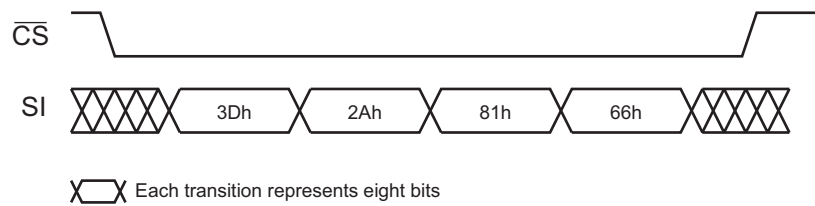
Figure 9-3. Quad Enable
