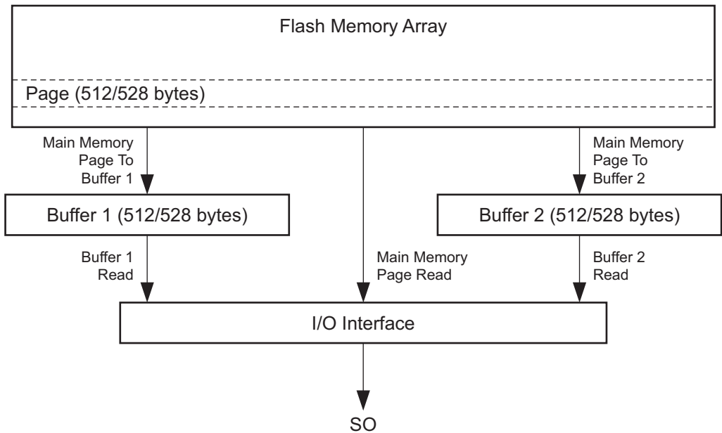
Figure 24-1. Block Diagram
