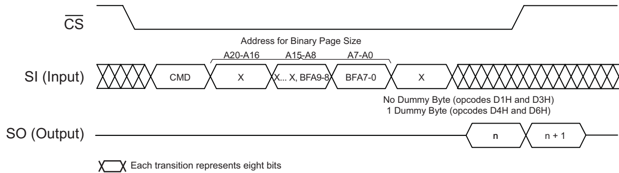
Figure 24-4. Buffer Read
