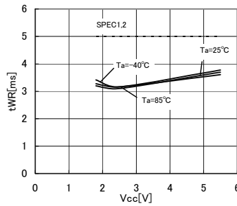
Fig.28 Internal write cycle time t_{WR}
