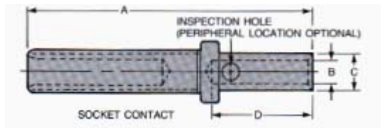
HDT-48-00 Universal Hand Crimp Tool Solid Contacts
