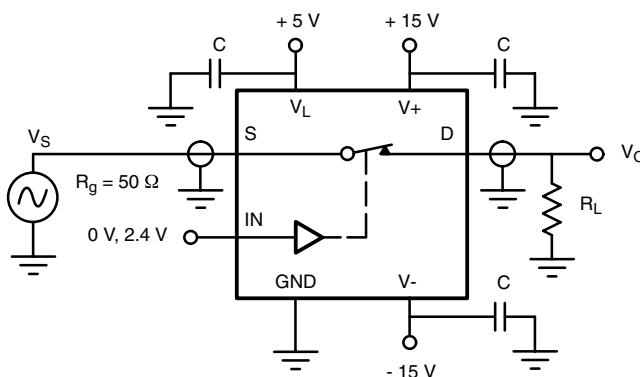
Figure 8. Insertion Loss
