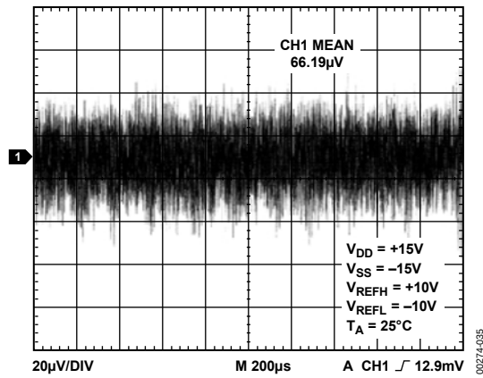
Figure 34. Broadband Noise
