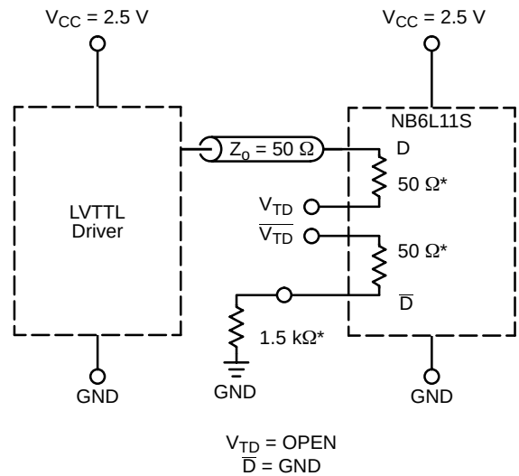
Figure 12. LVTTTL Interface
