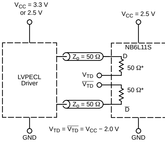
Figure 7. LVPECL Interface
