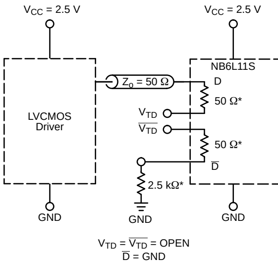
Figure 11. LVCMOS Interface
