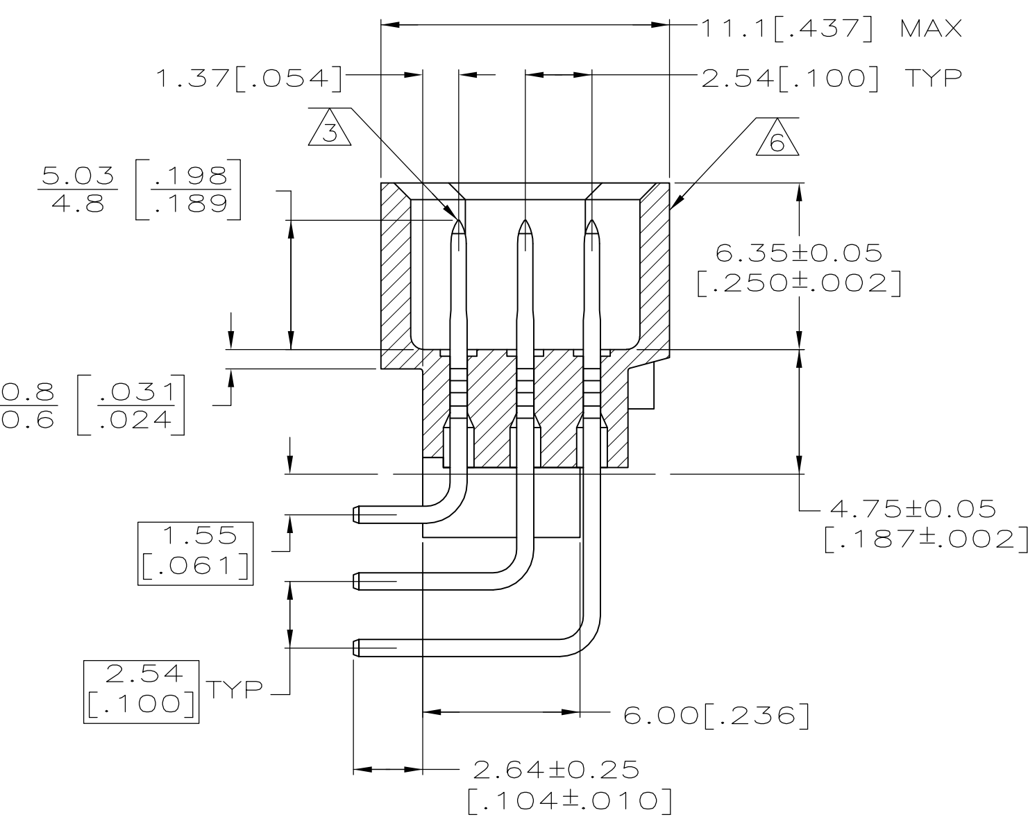
SECTION X-X
