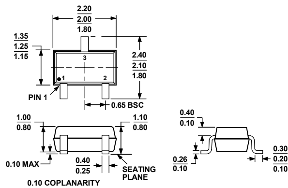
Figure 24. 3-Lead Thin Shrink Small Outline Transistor Package [SC70] (KS-3)
