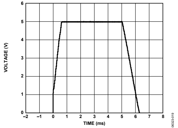
Figure 20. Large Signal Transient Response No Load, V_S = 5\text{ V}
