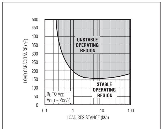
Figure 4. Capacitive-Load Stability
