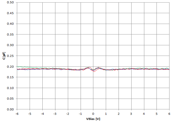
Figure 4. CV Characteristics
