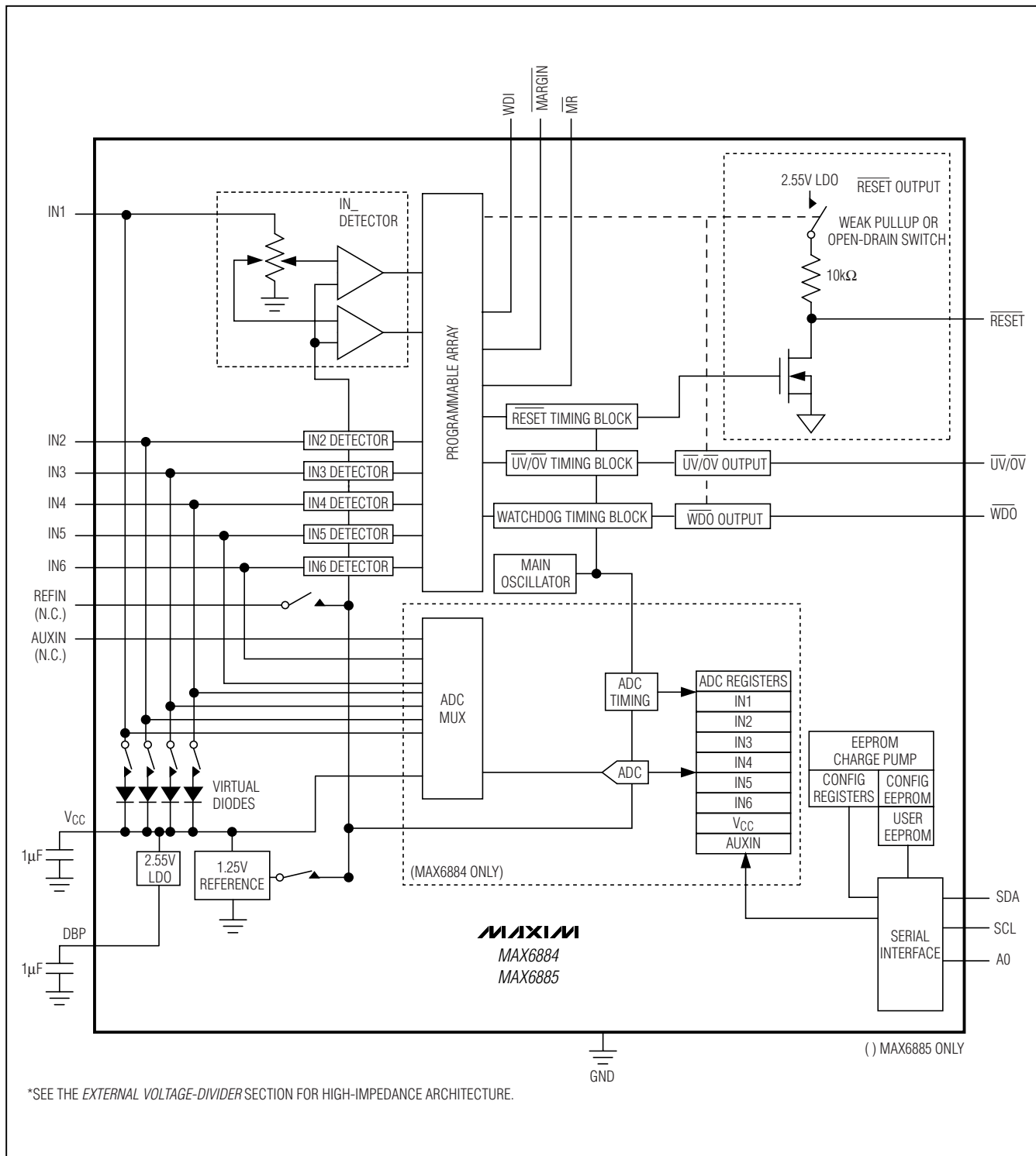
Functional Diagram
