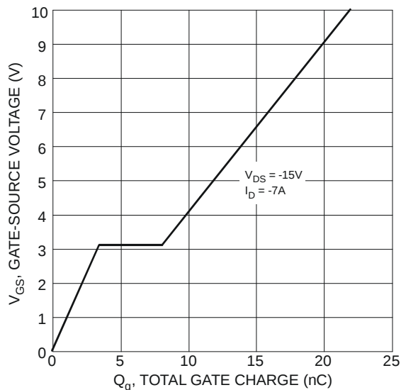
Figure 23 Gate-Charge Characteristics
