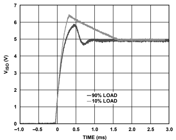
Figure 21. Typical Output Voltage Start-Up Transient at 10% and 90% Load, V_{ISO} = 5 V
