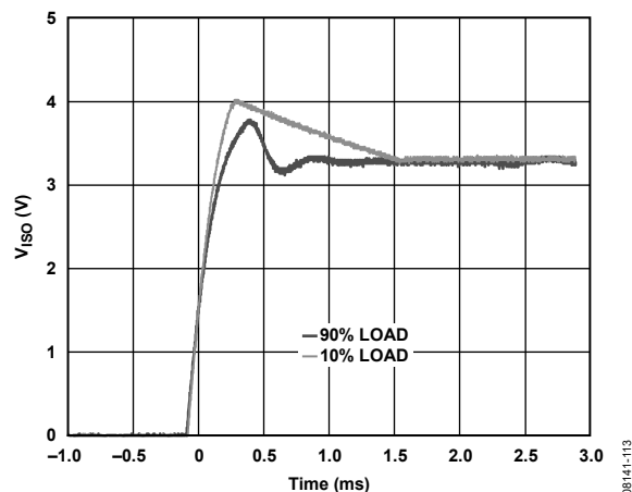
Figure 22. Typical Output Voltage Start-Up Transient at 10% and 90% Load, V_{ISO} = 3.3 V
