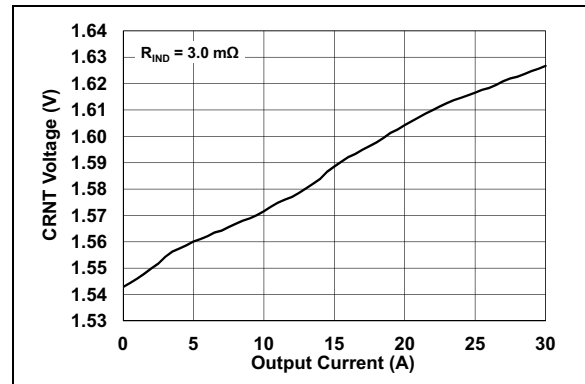
FIGURE 7-17: CRNT Voltage vs. Output Current.
