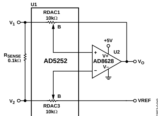
Figure 45. Current-Sensing Amplifier
