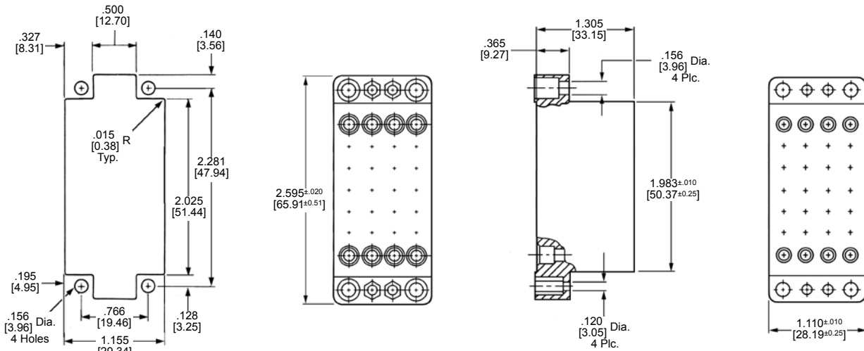
Plug Housing
