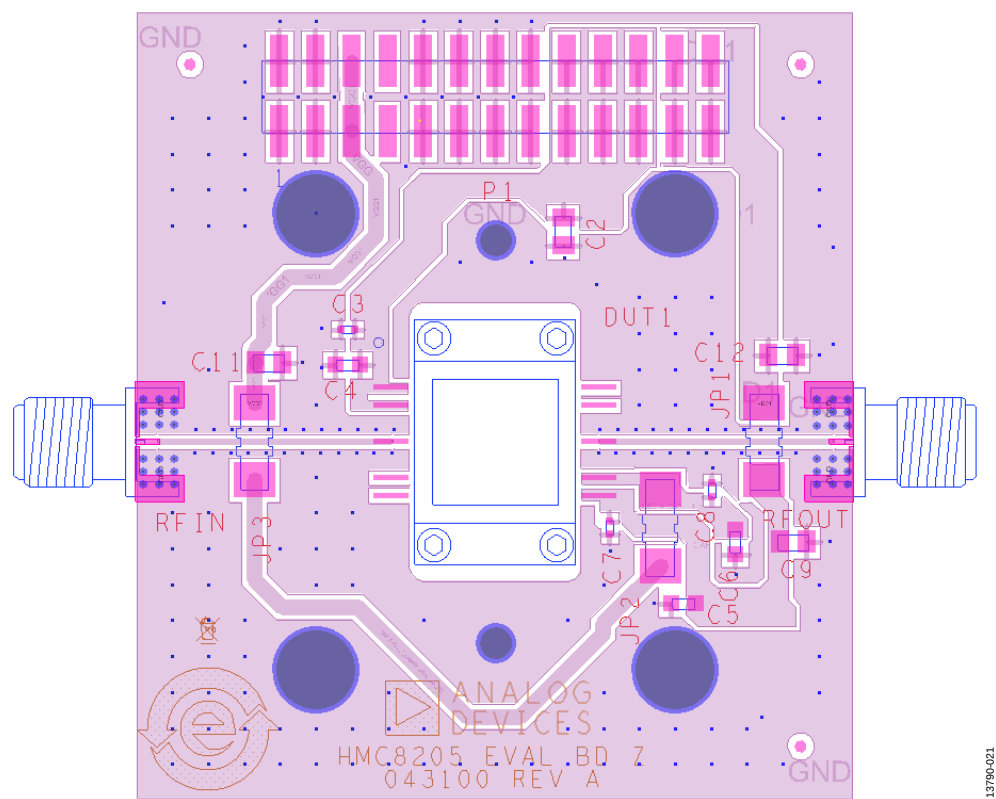
Figure 40. Evaluation PCB
