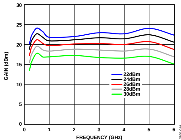
Figure 30. Gain vs. Frequency at Various Input Powers
