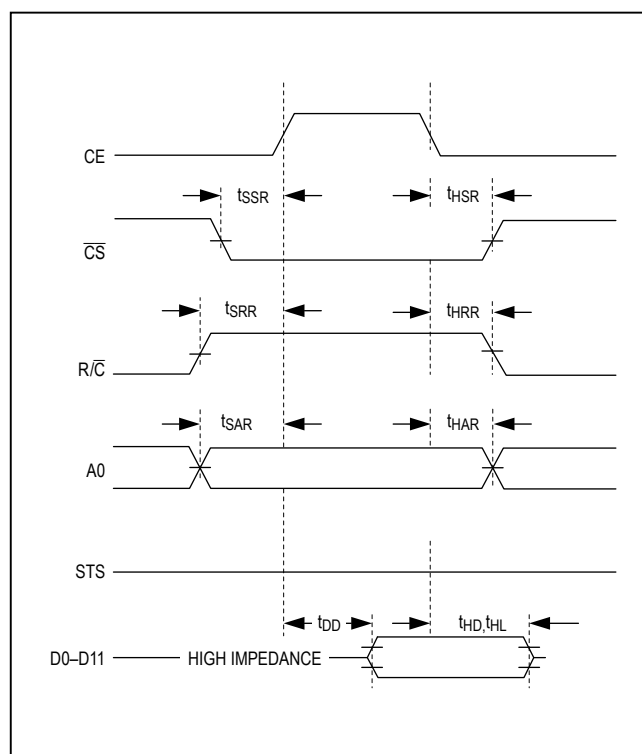
Figure 5. Read Timing
