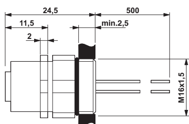
M12 flush-type socket, can be positioned
