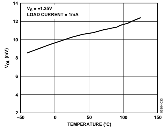
Figure 38. Output Voltage Swing Low vs. Temperature
