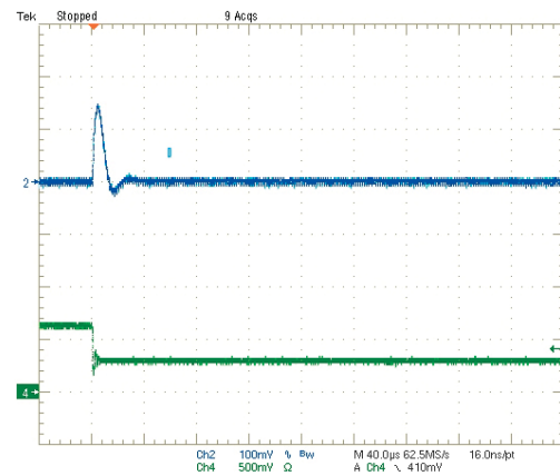
Step Load Transient Response (Vin=5V, Vout=0.6V, Cload=0, Iout=3A to 1.5A) Trace 2=Vout, 100 mV/div. Trace 4=Iout, 2.5A/div.
