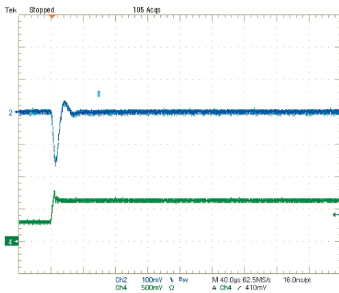
Step Load Transient Response (Vin=5V, Vout=0.6V, Cload=0, Iout=1.5A to 3A) Trace 2=Vout, 100 mV/div. Trace 4=Iout, 2.5A/div.
