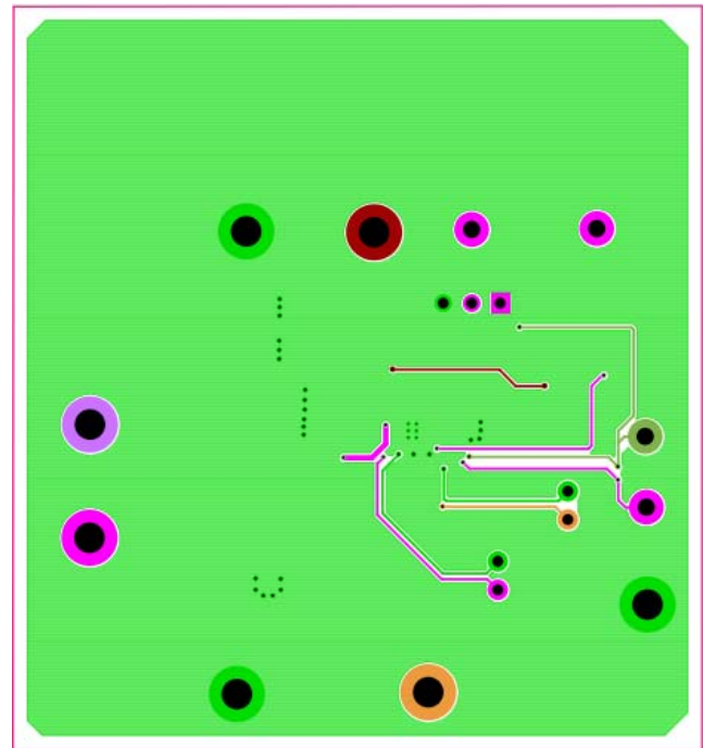
Figure 8. Bottom Layer
