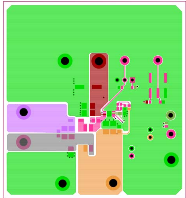
Figure 6. Top Layer
