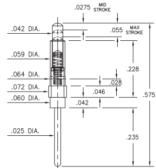
0929-0-15-20-75-14-11-0 Standard Stroke
