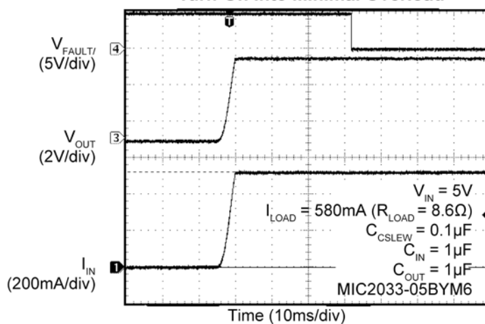
Turn-On Into Minimal Overload
