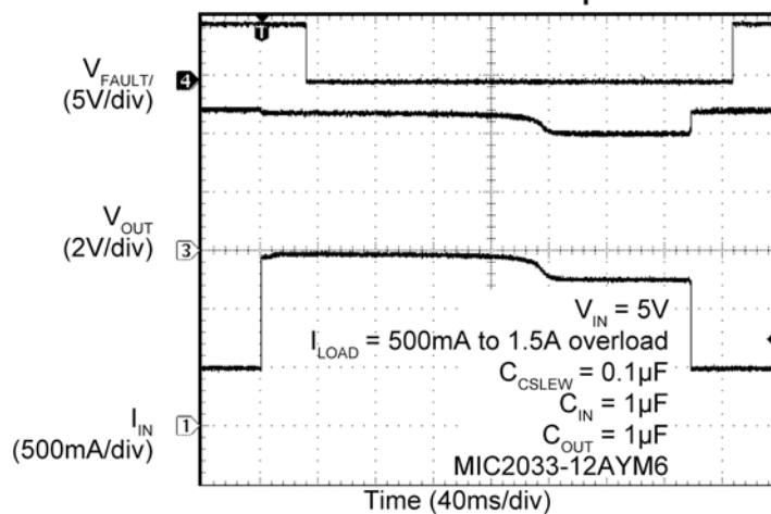
1.5A Overload Response
