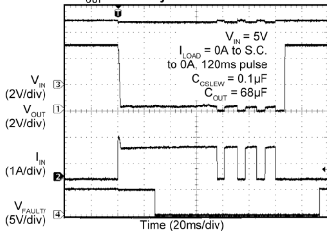
V_{\text{OUT}} Recovery from Thermal Shutdown
