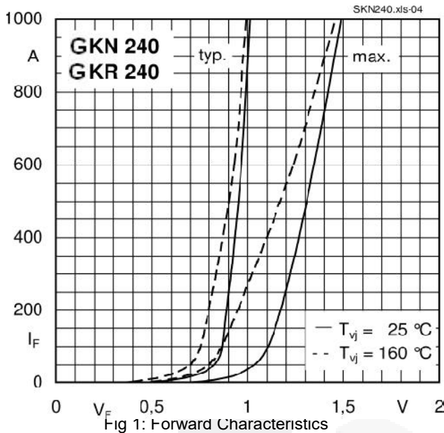
Fig 1: Forward Characteristics
