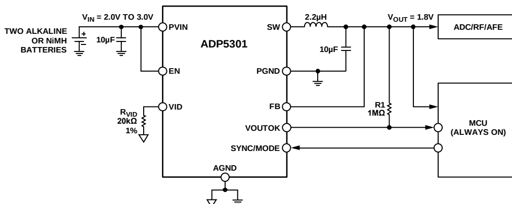
Figure 41. Typical ADP5301 Application with Two Alkaline/NiMH Batteries
