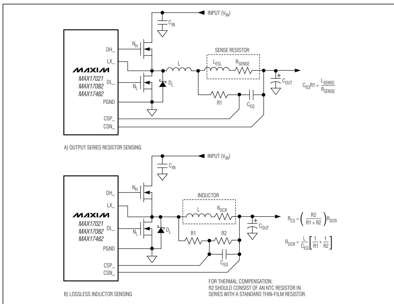
Figure 4. Current-Sense Methods
