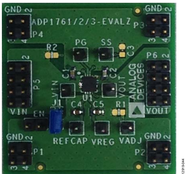
Figure 44. Evaluation Board
