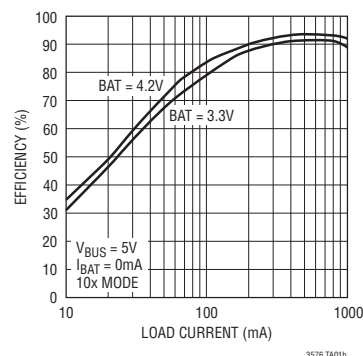
PowerPath Switching Regulator Efficiency to System Load ( P_{VOUT}/P_{VBUS} )
