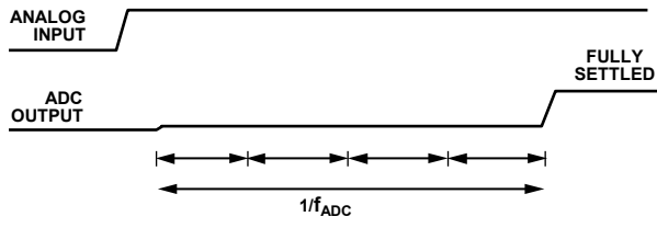
Figure 31. Sinc 4 Zero Latency Operation
