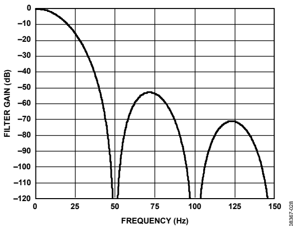
Figure 32. Sinc 4 Filter Response (FS[9:0] = 96)
