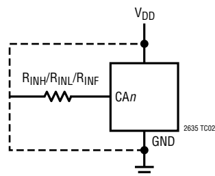
Test Circuit 2
