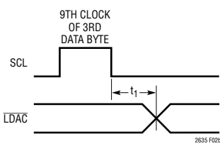
Figure 2b. LTC2635 LDAC Timing (QFN Package Only)
