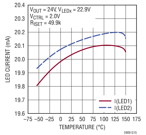
LED Current
