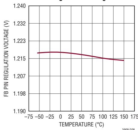
FB Pin Regulation Voltage
