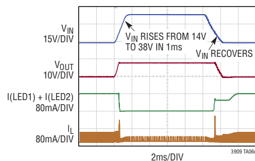
Protection in High V_{IN} Event
