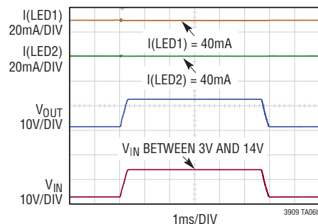
Protection in High V_{IN} Event
