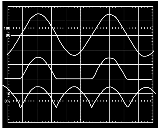
Figure 43. Single-Supply Half- and Full-Wave Rectifier
