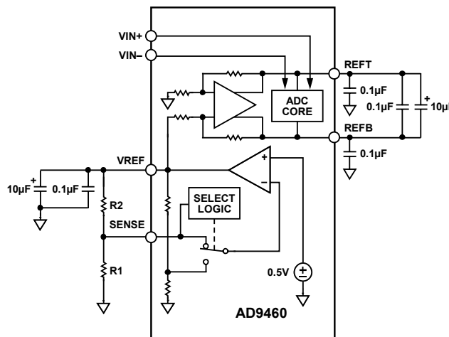
Figure 45. Programmable Reference Configuration
