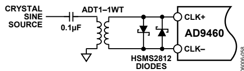
Figure 48. Crystal Clock Oscillator, Differential Encode
