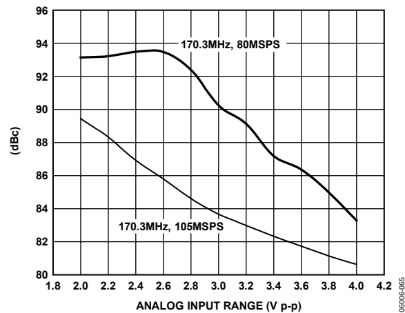
Figure 42. SFDR vs. Analog Input Range
