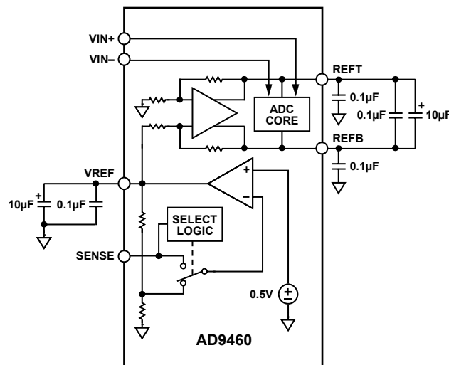
Figure 44. Internal Reference Configuration
