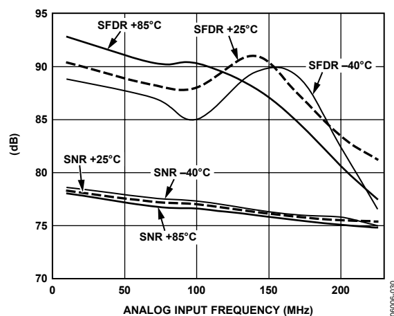
Figure 29. 80 MSPS, SNR/SFDR vs. Analog Input Frequency, 3.4 V p-p, CMOS Mode
