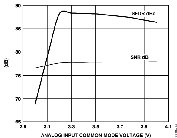
Figure 27. 105 MSPS, SNR/SFDR vs. Analog Input Common Mode
