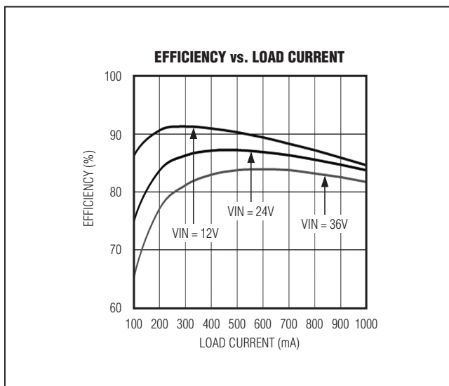
Figure 2. MAX17502E Efficiency
