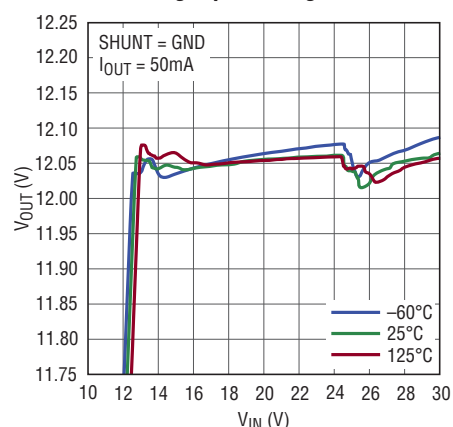
12V Output Voltage vs Falling Input Voltage
