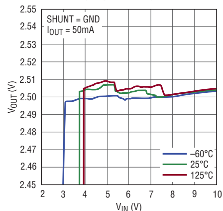
2.5V Output Voltage vs Falling Input Voltage
