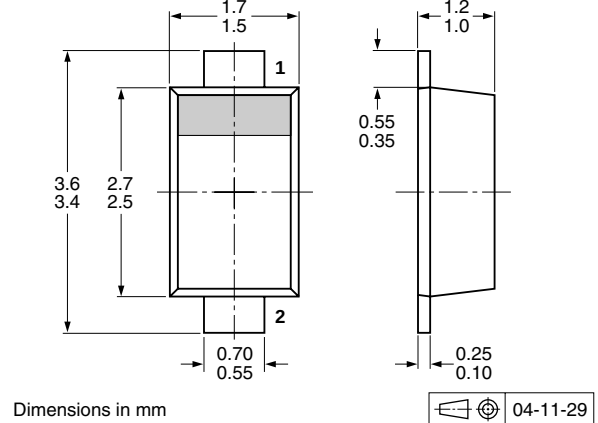
Fig 8. Package outline SOD123F
