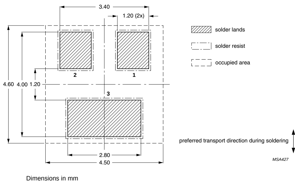
Fig 18. Wave soldering footprint SOT23 (TO-236AB)
