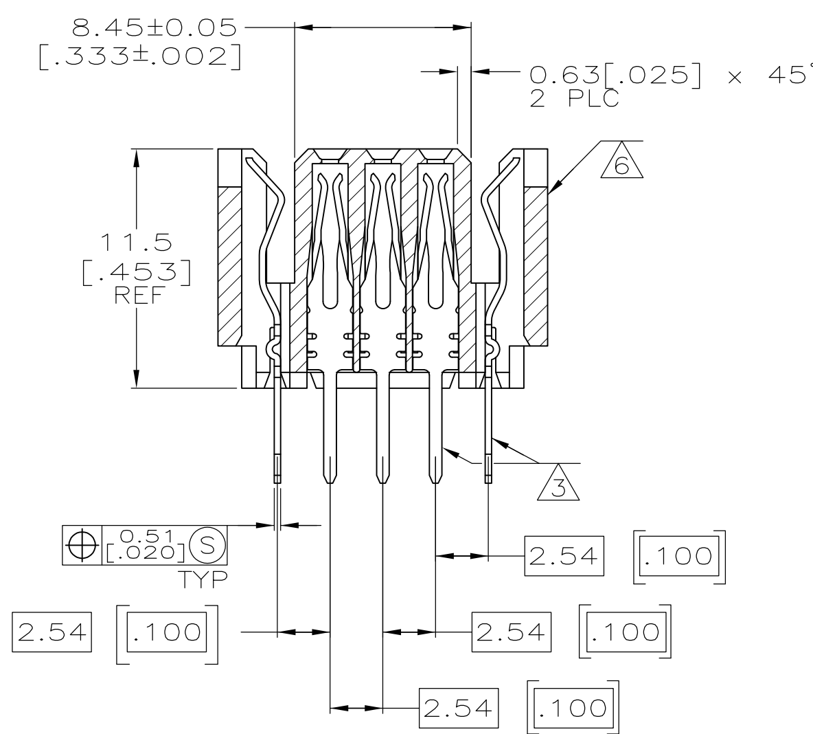
SECTION X-X
