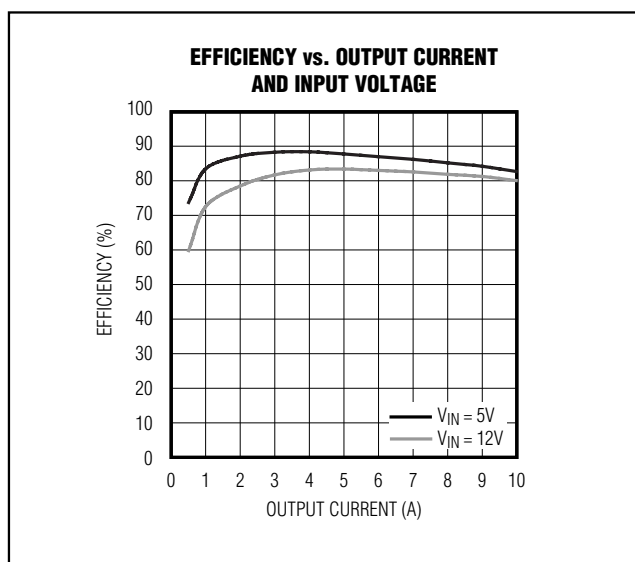
Figure 9. Efficiency vs. Output Current, Switching Frequency = 500kHz
