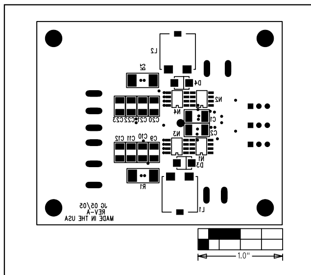
Figure 7. MAX5066 EV Kit Component Placement Guide—Solder Side
