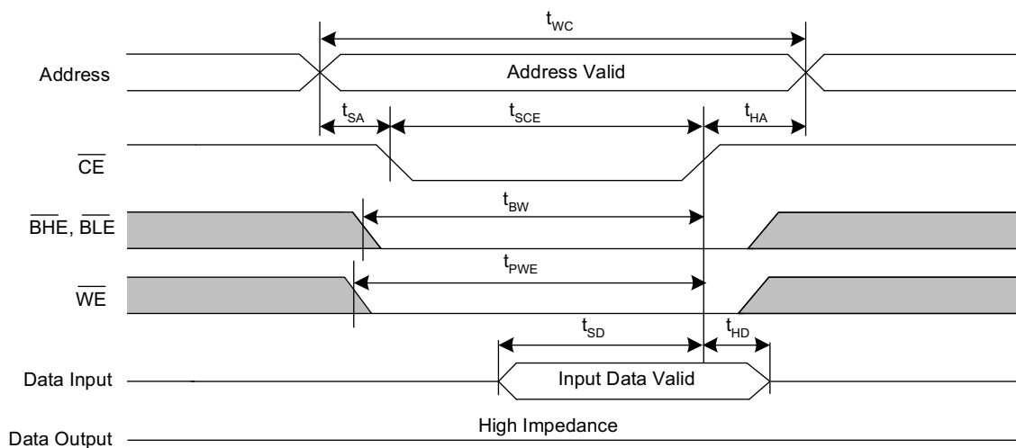
Figure 7. SRAM Write Cycle #2 ( \overline{\text{CE}} Controlled) [27, 28, 29, 30]
